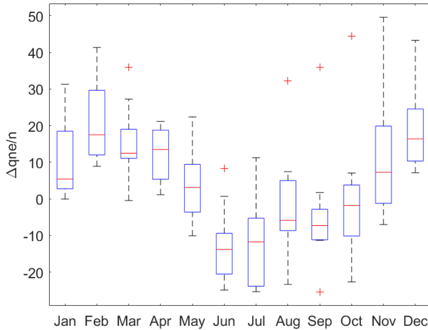
Figure 3.11. Changes in monthly average of the percentage of days that flow is less than environmental flow requirements ( qne/n ) for WPI calculation between the baseline and climate scenarios with the nine GCMs models
