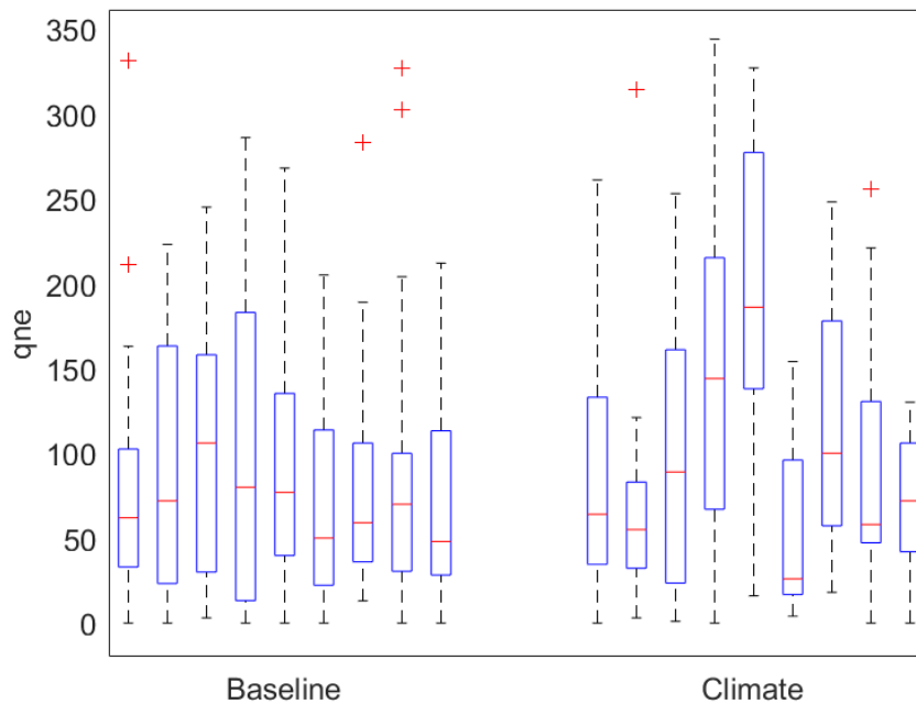
Figure 3.12. Inter-annual variations of the number of days that flow is less than environmental flow requirements ( qne ) under the baseline and climate scenarios with the nine GCMs models (each boxplot represents results with one climate model in order as Table 3.3.)
