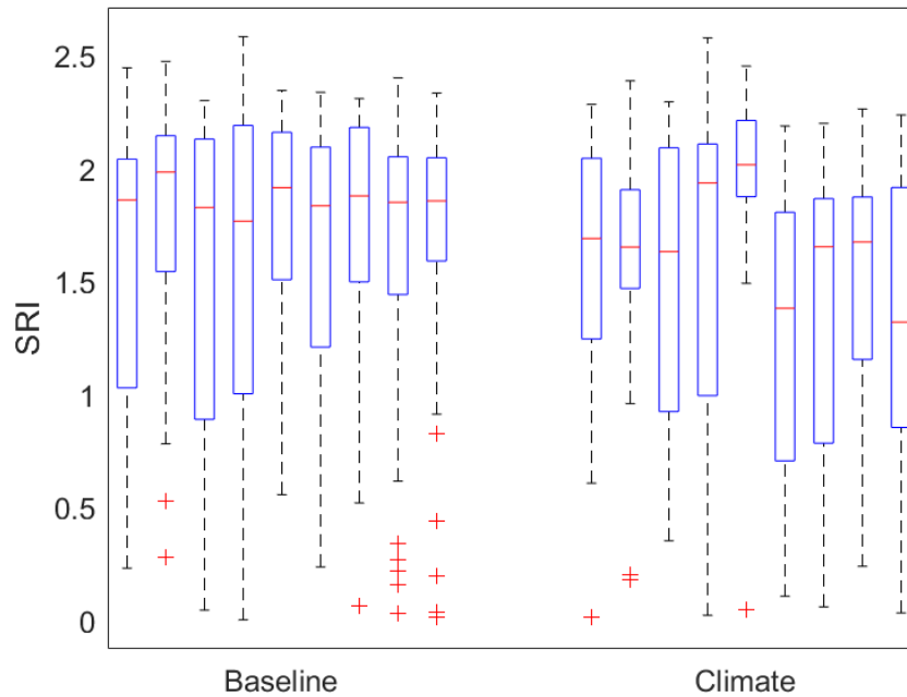
Figure 3.10. Inter-annual variations of the three ESs under the baseline and climate scenarios with the nine GCMs models (each boxplot represents results with one climate model in order as in Table 3.3. a: WPI; b: FRI; c: SRI)
